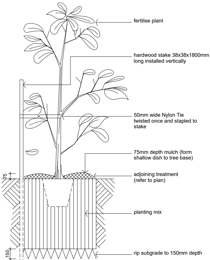
15-35 tree planting detail not to scale
