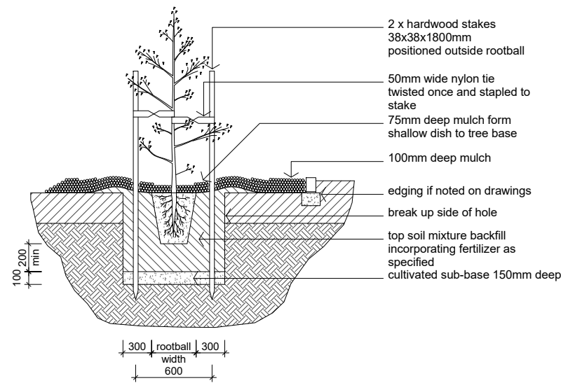
planting detail in garden beds
